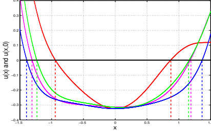
Fig. 7. An illustration of sets of p -safe initial states for Example 6. The states between the two dashed red curves are the 1-safe initial states falling within the computed robust invariant set. The states between the two dashed green curves are the 1-safe initial states falling within the computed backward reachable set with T = 1 . The states between the two dashed purple curves are the 1-safe initial states falling within the computed backward reachable set with T = 1.5 . The states between the two dashed blue curves are the (1 - 1.2 \times 10^{-6}) -safe initial states falling within the computed robust backward reachable set with T = 1 .
