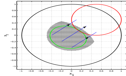
Fig. 6. An illustration of 0.8-safe initial states for Example 5 on the plane x_1 - x_2 with x_3 = x_4 = 0 . The black curve denotes the boundary of the set X . The red curve denotes the boundary of the set TR . The green curve denotes the boundary of the computed set of 0.8-safe initial states over the time horizon [0, T] . The gray region denotes the reach-avoid set corresponding to Eq. (20) with W_1(s, w_1) \equiv 0 and W_2(s, w_2) \equiv 0 . The blue curves denote trajectories of RODE (20) over time horizon [0, T] .
