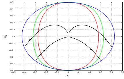
Fig. 10. An illustration of sets of p -safe initial states for Example 7 on the plane x_1 - x_7 with x_2 = x_3 = x_4 = x_5 = x_6 = 0 . The red curve denotes the boundary of the computed robust invariant set \overline{\text{TR}} . The green curve denotes the boundary of the computed inner-approximation \text{IN}' of 0.98-safe initial states. The blue curve denotes the boundary of the computed inner-approximation \text{IN} of the 0.98-safe initial states. The black curves denote the trajectories of RODE (21) in finite time.
