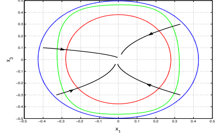
Fig. 9. An illustration of sets of p -safe initial states for Example 7 on the plane x_1 - x_3 with x_2 = x_4 = x_5 = x_6 = x_7 = 0 . The red curve denotes the boundary of the computed robust invariant set \overline{\text{TR}} . The green curve denotes the boundary of the computed inner-approximation \text{IN}' of 0.98-safe initial states. The blue curve denotes the boundary of the computed inner-approximation \text{IN} of the 0.98-safe initial states. The black curves denote the trajectories of RODE (21) in finite time.
