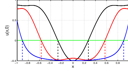
Fig. 3. An illustration of sets of p -safe initial states for Example 3. The states between the two dashed black lines, red lines and blue lines, are (1 - 1.2 \times 10^{-6}) -safe, 0.90-safe and 0.36-safe, respectively.
