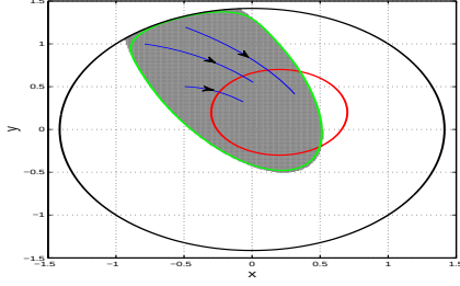
Fig. 4. An illustration of 0.9-safe initial states for Example 4. The black and red curves denote the boundary of the safe set X and the target set TR , respectively. The green curve denotes the boundary of the computed set of 0.9-safe initial states over the time horizon [0, T] . The gray region denotes the reach-avoid set corresponding to Eq. (19) with W(s, w) \equiv 0 . Blue curves denote trajectories of RODE (19) over the time horizon [0, T] .
