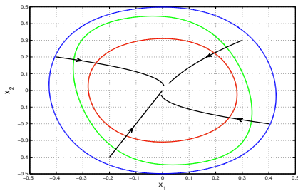
Fig. 8. An illustration of sets of p -safe initial states for Example 7 on the plane x_1 - x_2 with x_3 = x_4 = x_5 = x_6 = x_7 = 0 . The red curve denotes the boundary of the computed robust invariant set \overline{\text{TR}} . The green curve denotes the boundary of the computed inner-approximation \text{IN}' of 0.98-safe initial states. The blue curve denotes the boundary of the computed inner-approximation \text{IN} of 0.98-safe initial states. The black curves denote the trajectories of RODE (21) in finite time.
