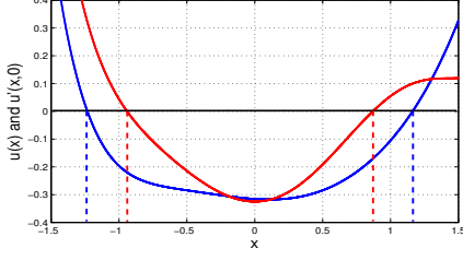
Fig. 2. An illustration of 1-safe initial states for Example 2. Red and blue solid curves denote u(x) and u'(x,0) , respectively. The computed robust invariant set TR is the set of states between the two dashed red lines. The computed inner approximation IN of the robust backward reachable set over the time horizon [0, \tau] is the set of states between the two dashed blue lines.
