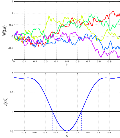
Fig. 1. An illustration of the computed p -safe initial states for Example 1. Above: Five sample paths of the Wiener process over the time horizon [0, T] are presented. Below: The solid blue curve denotes u(x, 0) computed by solving (11). The computed p -safe initial states are the states between the two dashed blue lines, i.e., \text{IN} = \{x \in X \mid u(x, 0) \leq 0\} .
